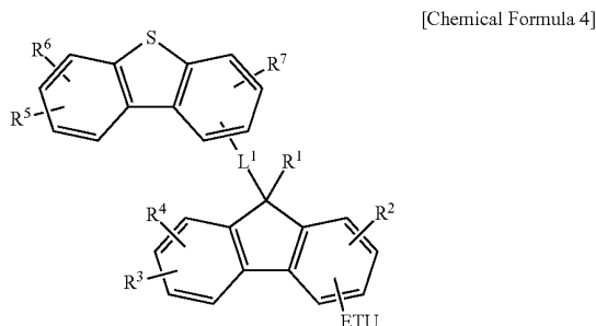
[Chemical Formula 4]
