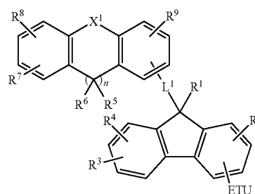
[Chemical Formula 3]
