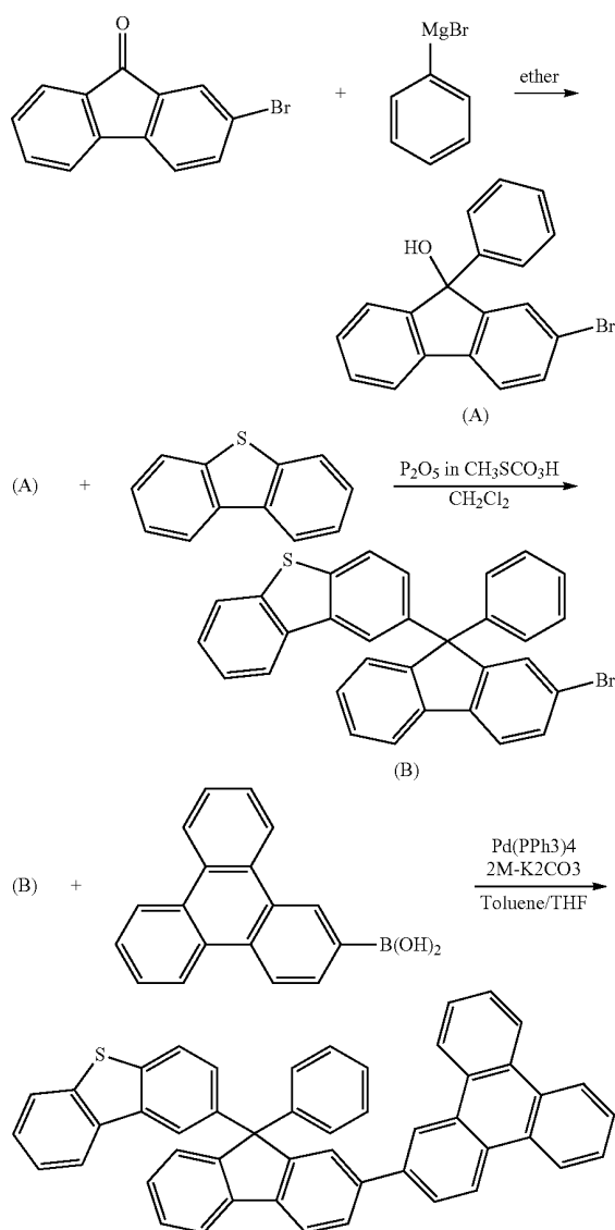
[Reaction Scheme 1]
