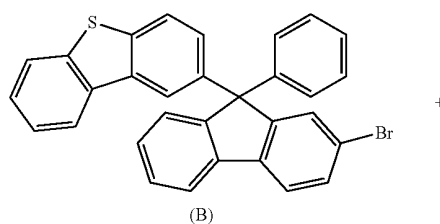
[Reaction Scheme 2]
